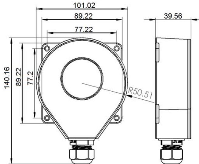
Figure 1 – Detector Dimensions
