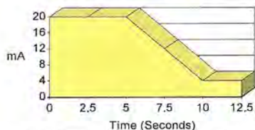
Fig. 5 Typical Response after last Flame seen - IR Flame Sensor
