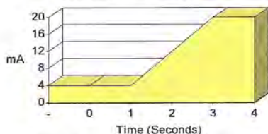
Fig. 4 Typical Response on seeing Flame - IR Flame Sensor
