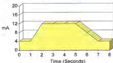
Fig. 6 Typical Response to Burst of Flame - IR Flame Sensor
