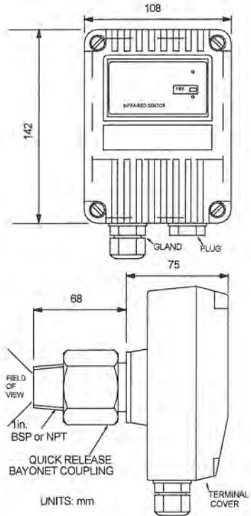
Fig. 8 Dimensions – IR Flame Sensor
