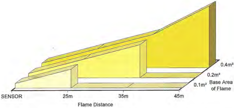
Fig. 2 Sensor centre line detection range for n-heptane fire (yellow sooty flame) - IR Flame Sensor, sensitivity set high for class 1 performance
